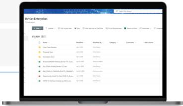
MS SharePoint
